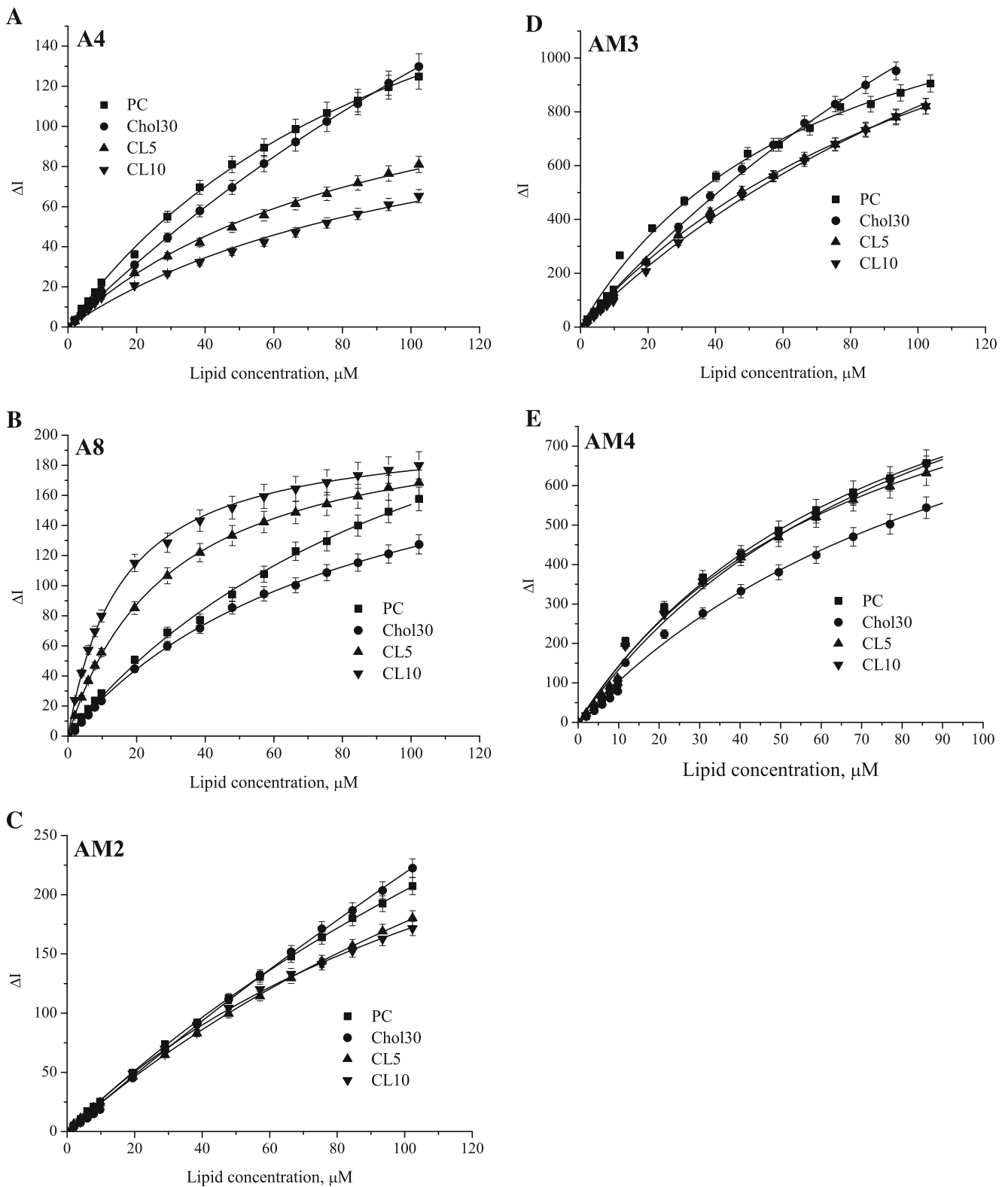
Fig. 3 Isotherms of aminobenzanthrone binding to model lipid membranes. Dye concentration was 1.0 μM (a), 1.6 μM (b), 2.0 μM (c), 3.5 μM (d), 1.2 μM (e)
